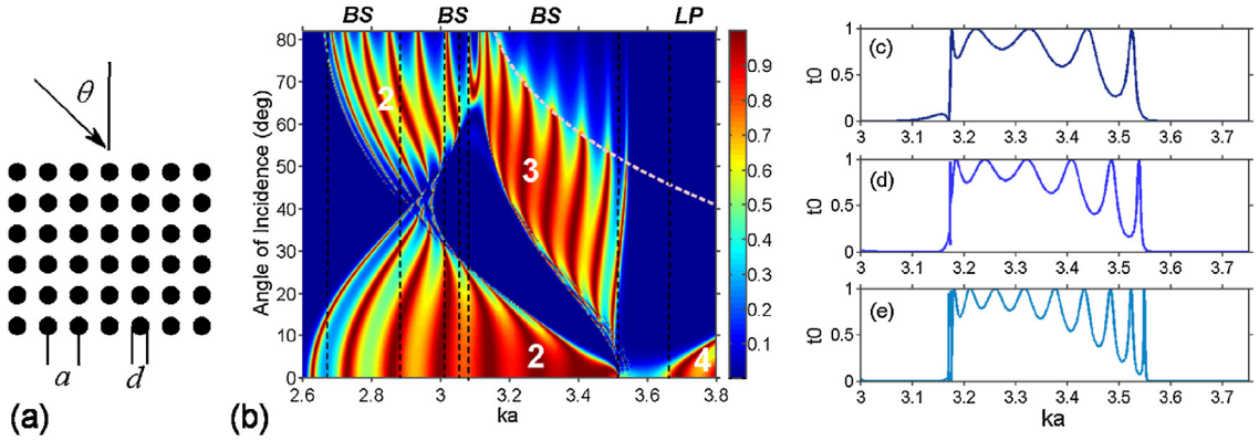
Fig. 2. (a) General geometry used in transmission studies; (b) Map of t_0 in (ka, \theta) -plane at d/a=0.443 , \epsilon=9.61 , and N=8 ; straight vertical lines – approximate boundaries of ka -ranges that can be used for bandstop (BS) and low-pass (LP) spatial filtering, dashed curve – threshold line for the diffraction order m=-1 ; large numbers, 2, 3 and 4, indicate transmission area due to the corresponding Floquet–Bloch mode; (c–e) t_0 vs ka at d/a=0.443 , \epsilon=9.61 , \theta=47^\circ , and (c) N=6 , (d) N=8 , and (e) N=12 .
