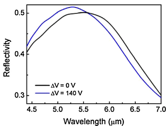
Fig. 3. Calculated reflectance spectra at different \Delta V .
