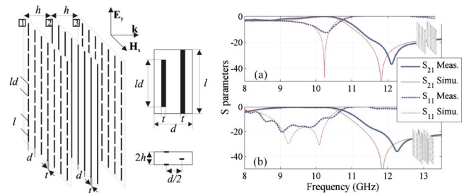
FIG. 1. (Color online) Schematic representation of the metasurface, and unit cell geometry: top and lateral views. Right panel: the simulated and measured transmission and reflection spectra through (a) the double grid of cutwires and (b) in the presence of the continuous wires.
