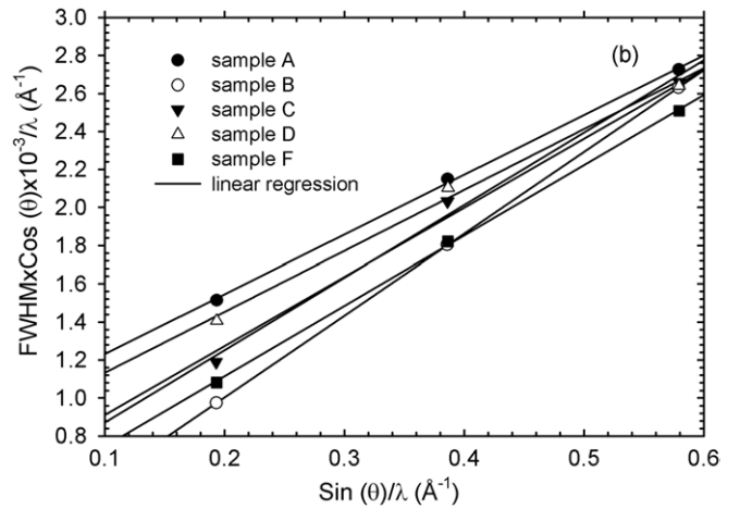
Figure 6. Williamson–Hall plot for GaN layers for all samples. (a) Triple-axis \omega scan and (b) triple-axis \omega - 2\theta scan were measured for the (000 l ) ( l = 2, 4, 6 ) reflections indicated in the figure. The lines result from a linear fit of the data.
